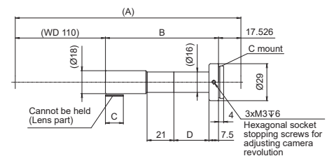
SE-110ST20/SE-110ST40 (Straight)
