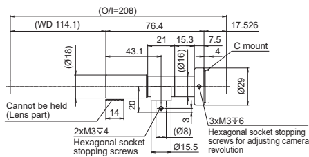
SE-110VT15 (Coaxial)
