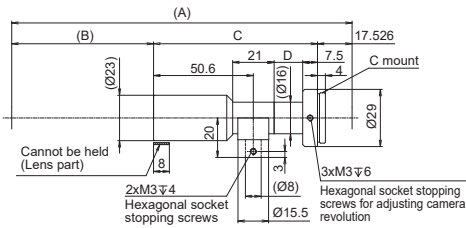
SE-110VT08/SE-110VT10 (Coaxial)
