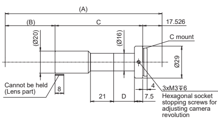
SE-65ST08/SE-65ST10 (Straight)
