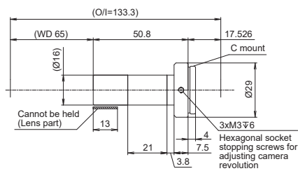
SE-65ST15 (Straight)
