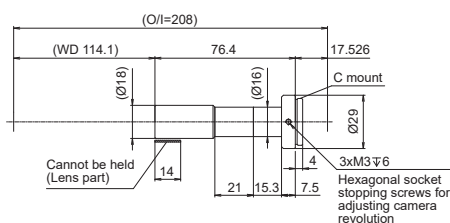
SE-110ST15 (Straight)
