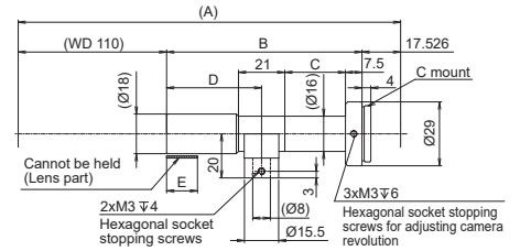
SE-110VT20/SE-110VT40 (Coaxial)
