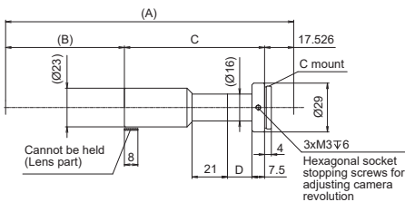
SE-110ST08/SE-110ST10 (Straight)
