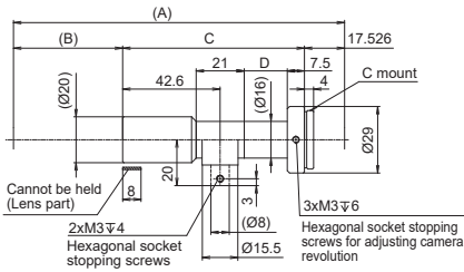
SE-65VT08/SE-65VT10 (Coaxial)
