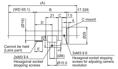
SE-65VT20/SE-65VT40 (Coaxial)
