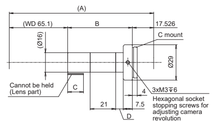
SE-65ST20/SE-65ST40 (Straight)
