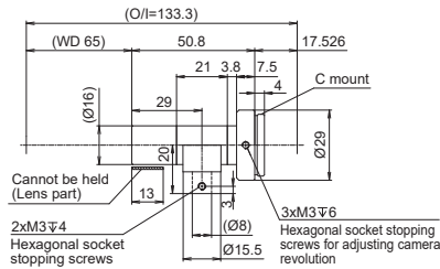
SE-65VT15 (Coaxial)
