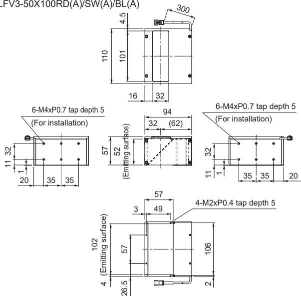
LFV3-50X100RD(A)/SW(A)/BL(A)
