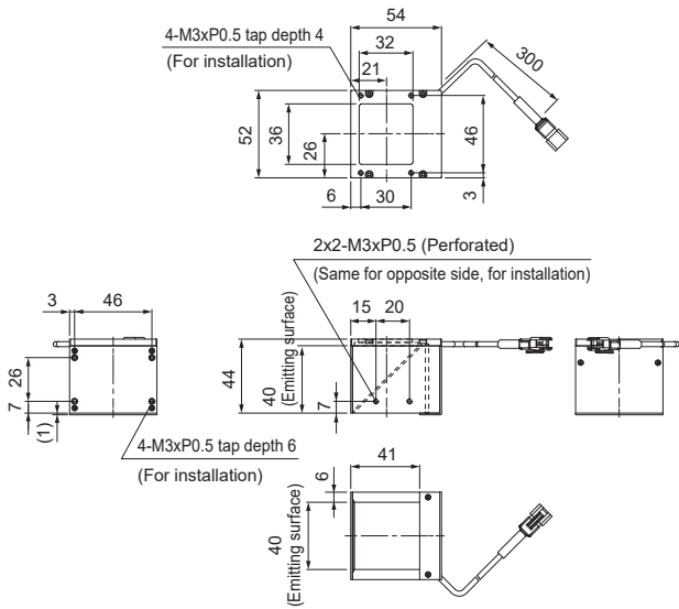
LFV3-40RD(A)/SW(A)/BL(A)
