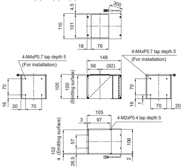
LFV3-100RD(A)/SW(A)/BL(A)
