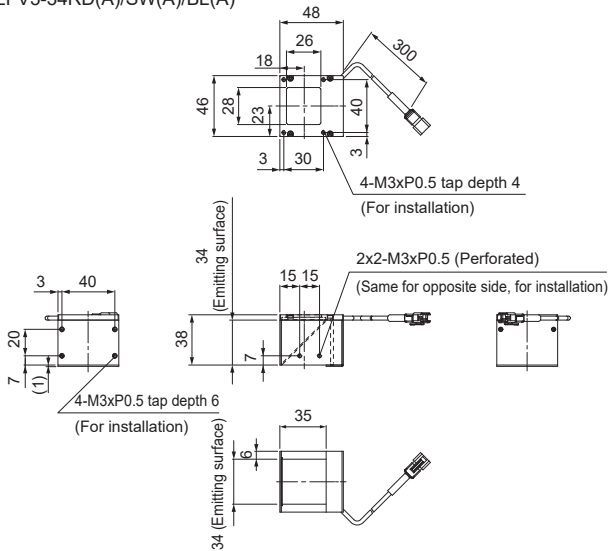
LFV3-34RD(A)/SW(A)/BL(A)
