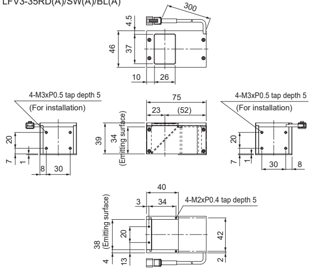
LFV3-35RD(A)/SW(A)/BL(A)
