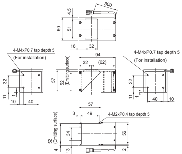
LFV3-50RD(A)/SW(A)/BL(A)
