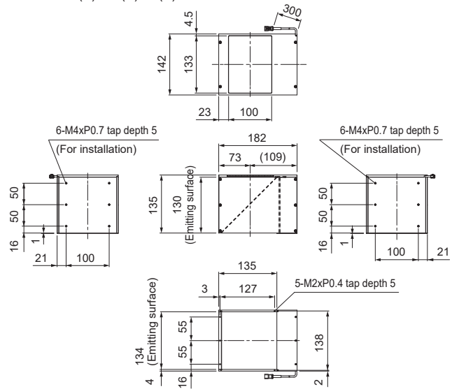
LFV3-130RD(A)/SW(A)/BL(A)
