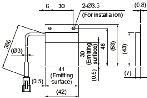
LFL-1012RD2-P / SW2-P / BL2-P / GR2-P
