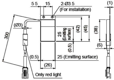
LFL-612RD2-P / SW2-P / BL2-P / GR2-P
